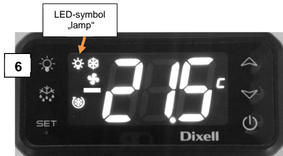
Fig. 3.1 Controller type DIXELL operating elements and display indicators (symbol)
